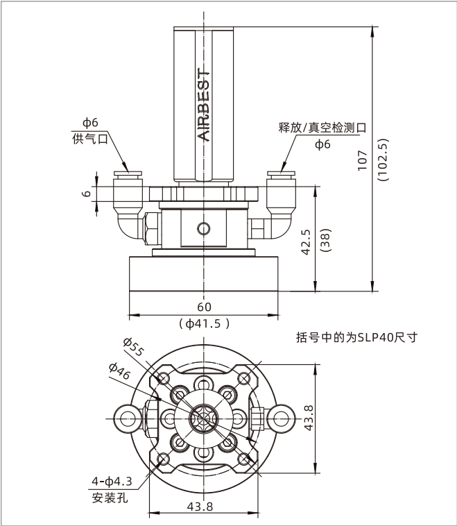
SLP60(40)-M10SD-F1
