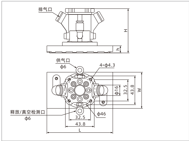
SLW100PK-M10Y-F1
