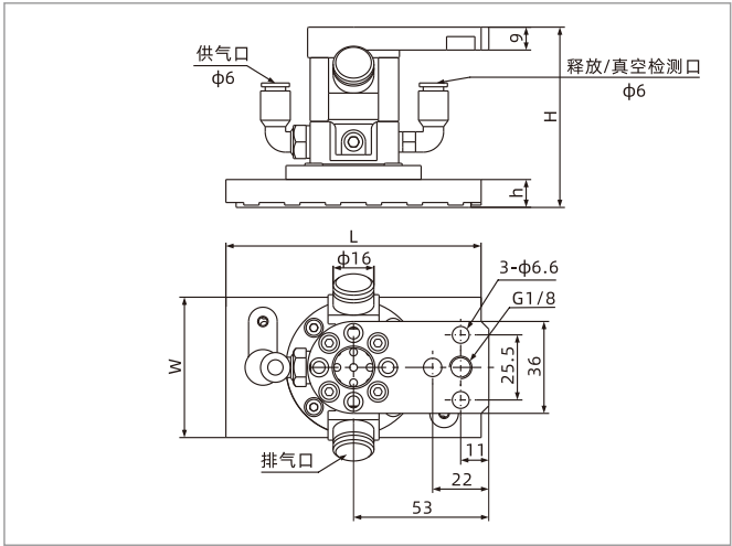
SLW115PK-M10Y-F3
