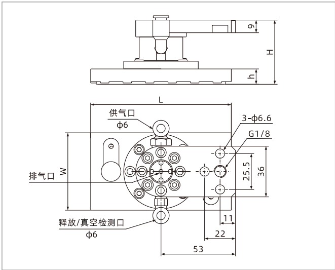
SLW□PK-M10I-F3
